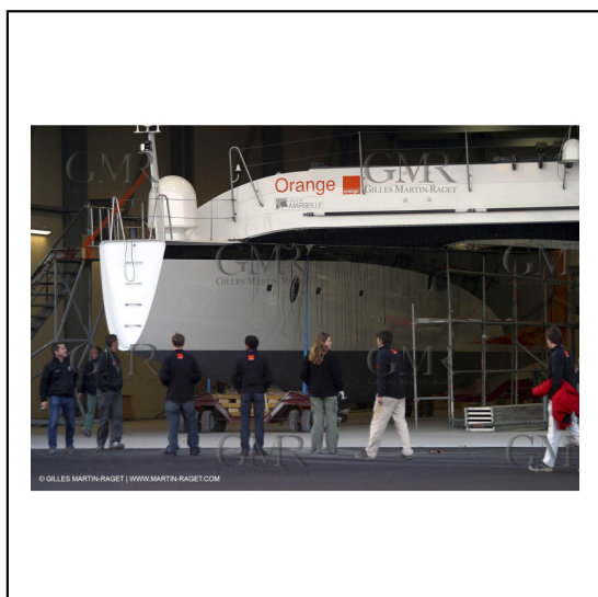
Vannes - Chantier Multiplast - sortie de chantier Orange II *** Vannes - Multiplast Boatyard - Orange II going out of the shed
