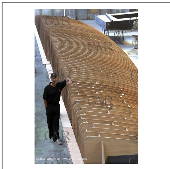
Vannes - Chantier Multiplast - Moules Orange II *** Vannes - Multiplast Boatyard - Orange II plugs
