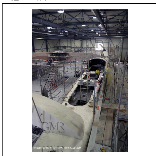
Vannes - Chantier Multiplast - Construction Orange II *** Vannes - Multiplast Boatyard - Orange II construction
