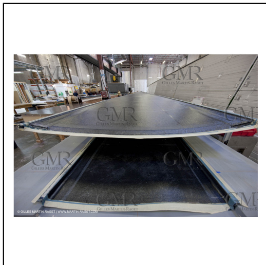
11/07/2009 - Anacortes (USA,CA) -33rd America's Cup - BMW ORACLE Racing - Wing construction at Core Builders***11/07/2009 - Anacortes (USA,CA) -33rd America's Cup - BMW ORACLE Racing - Wing construction at Core Builders
