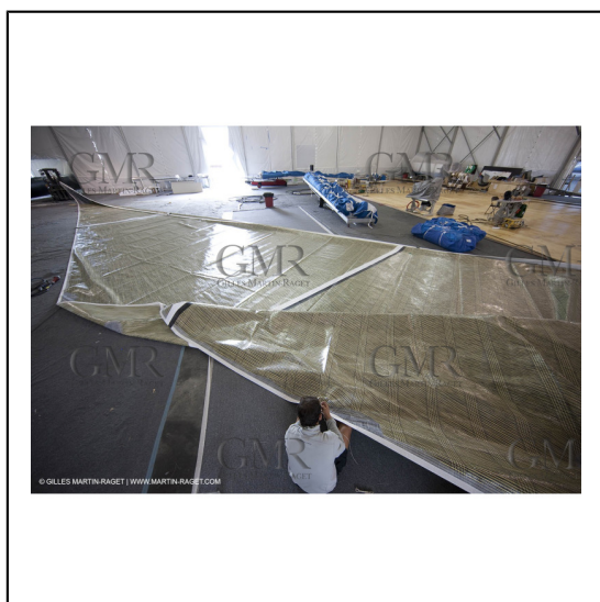
26/08/2008 - Anacortes (WA, USA) - America's Cup - BMW ORACLE Racing - 90 ft trimaran launch - structural tests completed by design team***26/08/2008 - Anacortes (WA, USA) - America's Cup - BMW ORACLE Racing - 90 ft trimaran launch - structural tests completed by Design Team
